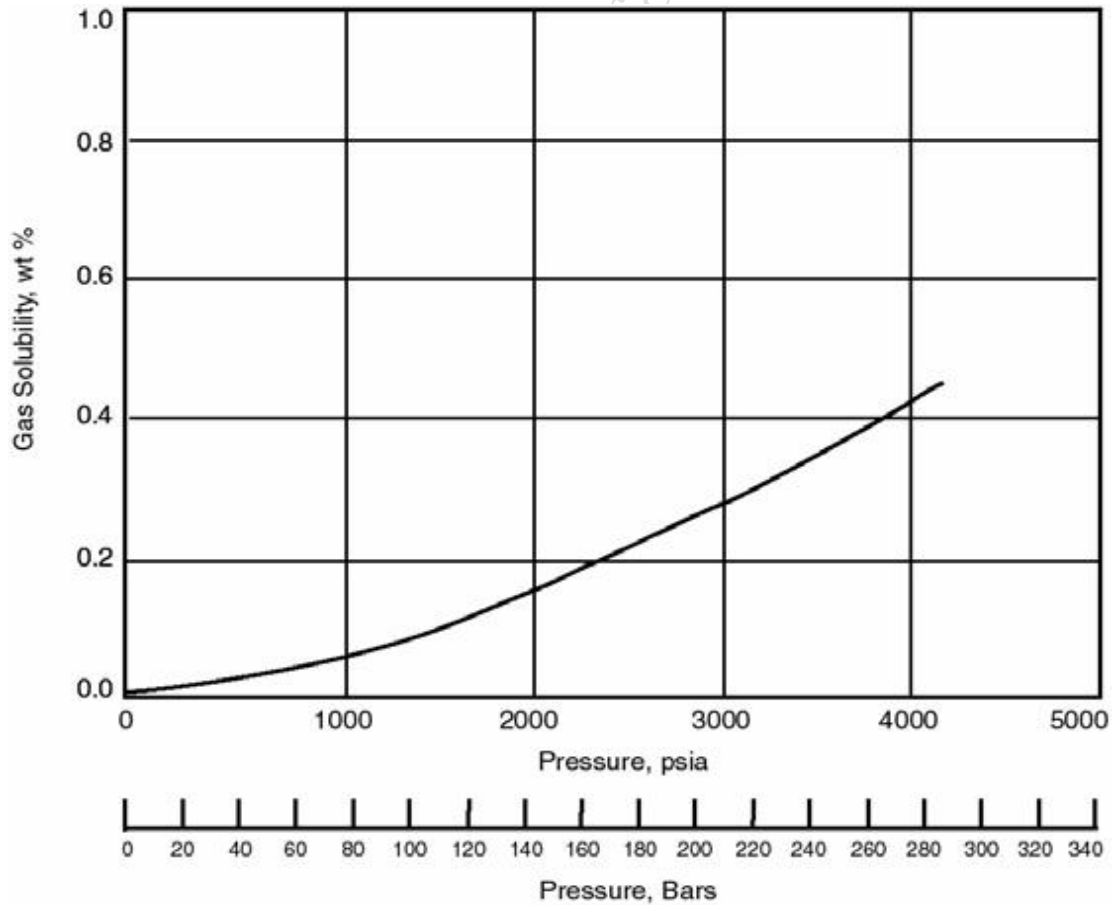
Figure 2 • Solubility of Hydrogen at 50°C (122°F) in UCON Compressor Lubricant R-4
